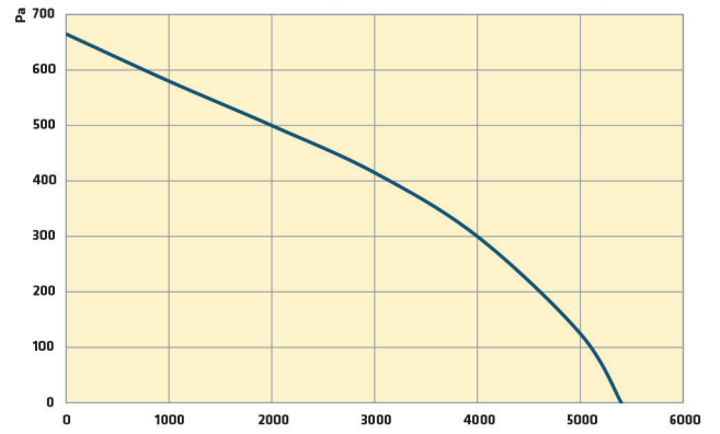
T/AXB-F 1300x650 T4 1,43 kW
