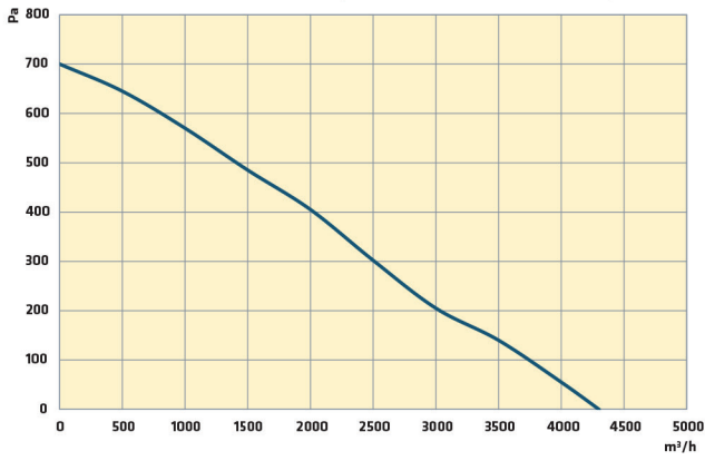
T/AXB-F 900x650 T4 1,43 kW
